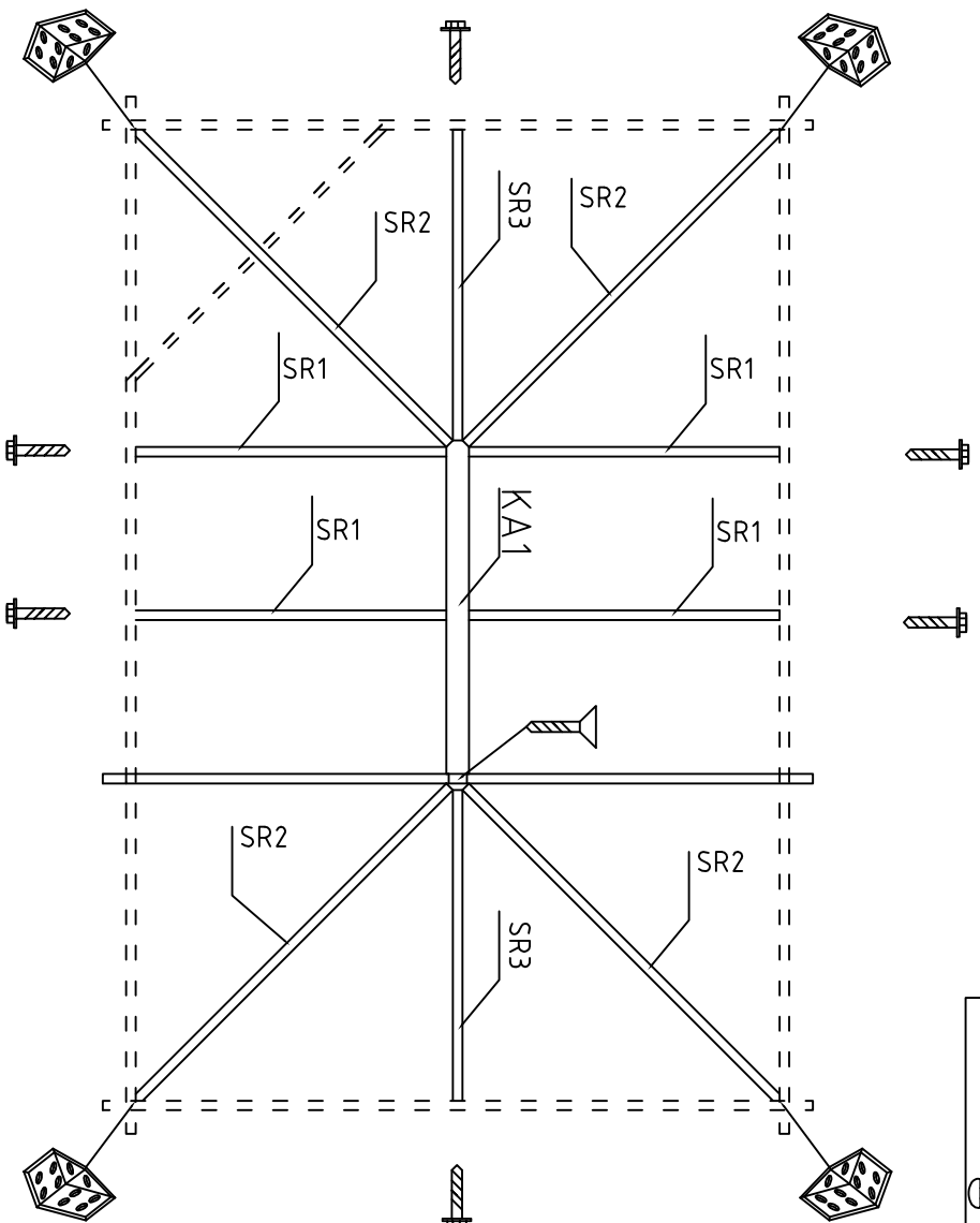
Dachbalken 40x58 (SR1) Montage
